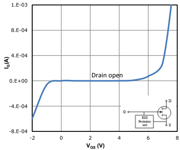
Fig 10: Typ. Gate-to-Source leakage
