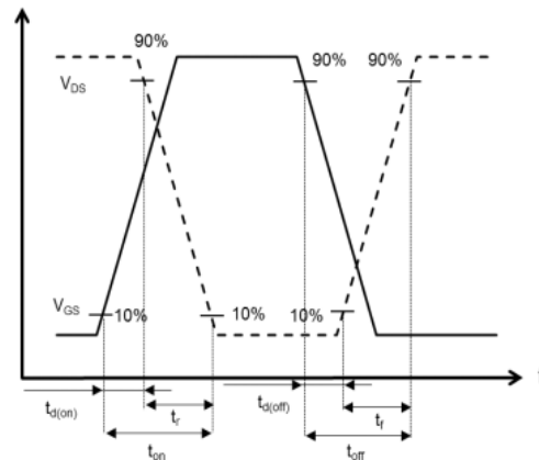
Figure 23 Typ.Switching times waveform
